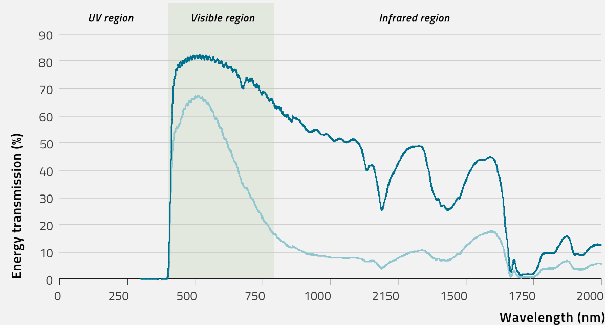
Electromagnetic spectrum of soda-lime float glass vs low iron soda-lime float glass 56mm bullet-resistant glass (Stanag 2)
