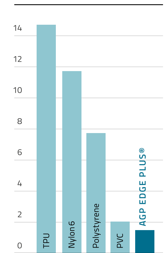
Water grams / 24 hours 1mm thickness / 100 in² area / 100°F / 90%
